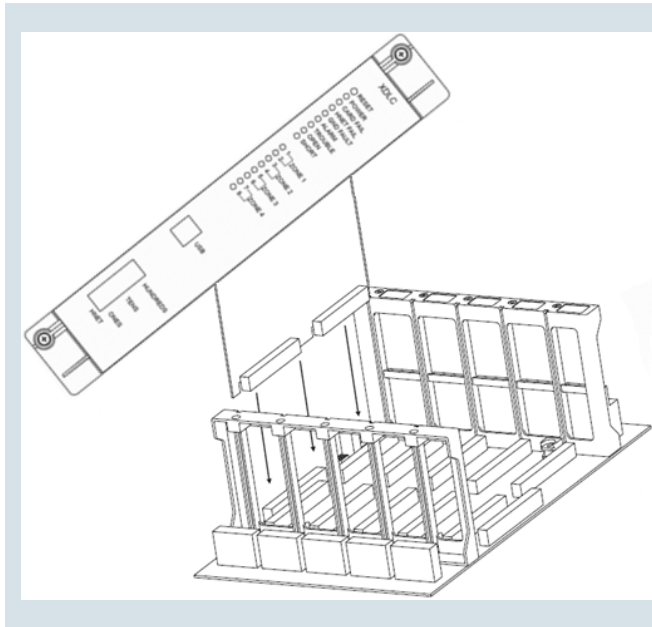
Model XDLC Diagram of an 'Class X' Device Loop Card mounted to a Siemens Card Cage
